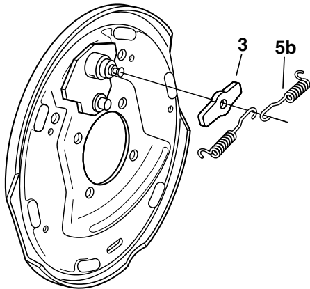
Before 3/18: Dual Retractor Spring Components
