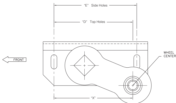
Chart 2 Bracket Dimensions
