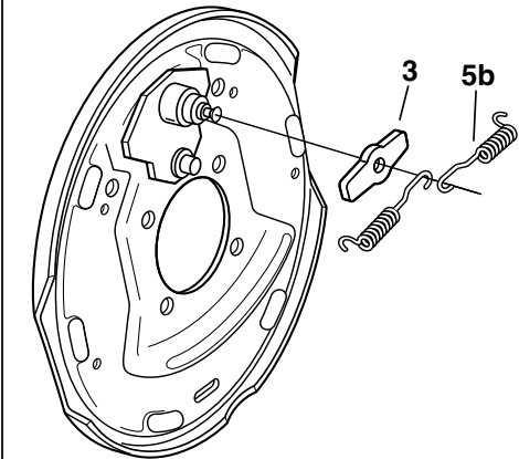
Before 3/18: Dual Retractor Spring Components
